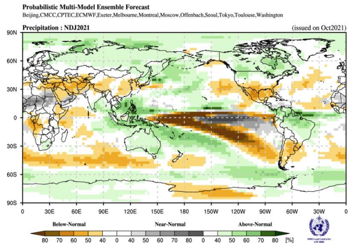
Figure 1. Probabilistic forecasts of surface air temperature and precipitation for the season November-January 2021-22. The tercile category with the highest forecast probability is indicated by shaded areas. The most likely category for below-normal, above-normal and near-normal is depicted in blue, red and grey shadings respectively for temperature, and orange, green and grey shadings respectively for precipitation. White areas indicate equal chances for all categories in both cases. The baseline period is 1993-2009.
