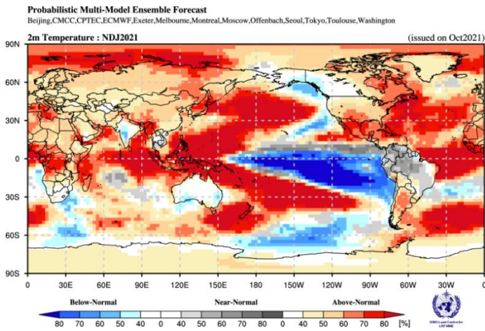
Figure 1. Probabilistic forecasts of surface air temperature and precipitation for the season November-January 2021-22. The tercile category with the highest forecast probability is indicated by shaded areas. The most likely category for below-normal, above-normal and near-normal is depicted in blue, red and grey shadings respectively for temperature, and orange, green and grey shadings respectively for precipitation. White areas indicate equal chances for all categories in both cases. The baseline period is 1993-2009.
