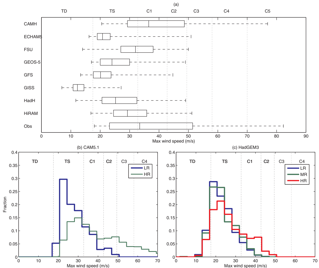
Figure 8. (a) Distributions of TC maximum intensity in models and observations. The vertical line shows the median of each distribution, the left and right edges of the box represent the 75th and 25th percentiles, respectively, and the whiskers extend to the maximum and minimum values in each case. Histograms of TC maximum intensity for (b) two horizontal resolutions of the CAM5.1 model and (c) three model resolutions of the HadGEM1 model. The vertical lines show the boundaries of the Saffir-Simpson hurricane classification scale. TD: Tropical Depression, TS: Tropical Storm, C1–C5: Category 1–5 hurricanes. LR: Low resolution, MR: Medium resolution, HR: High resolution.
