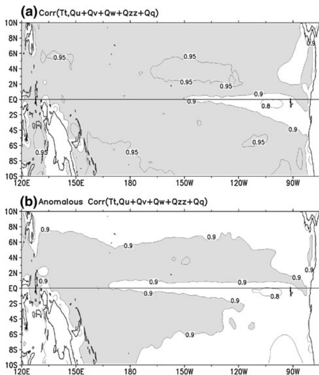
Fig. 2 Correlation coefficients between a T_t and Q_u + Q_v + Q_w + Q_q + Q_{zz} , and b Anomalous T_t and Q_u + Q_v + Q_w + Q_q + Q_{zz} . Contours are 0.8, 0.9, and 0.95. Contour values of 0.9 or higher are shaded
