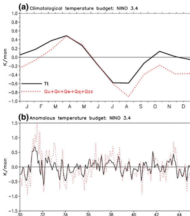
Fig. 12 Same as Fig. 3 except for temperature budget calculated using monthly averaged variables. The correlation coefficient between T_t and the forcing ( Q_u + Q_v + Q_w + Q_{zz} + Q_q ) is 0.92 and 0.74 in (a) and (b), respectively
