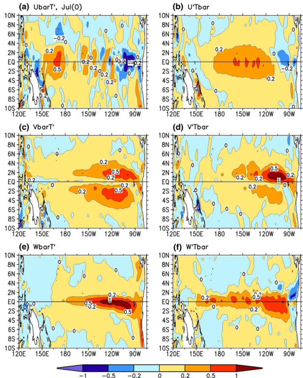
Fig. 8 Temperature budget distributions in Jul of year 0. a -\bar{u}T'_x , b -u'T_{\bar{x}} , c -\bar{v}T'_y , d -v'T_{\bar{y}} , e -\bar{w}T'_z , and f -w'T_{\bar{z}} . Contours are 0, \pm 0.2 , \pm 0.5 , and \pm 1^\circ\text{C mon}^{-1}
