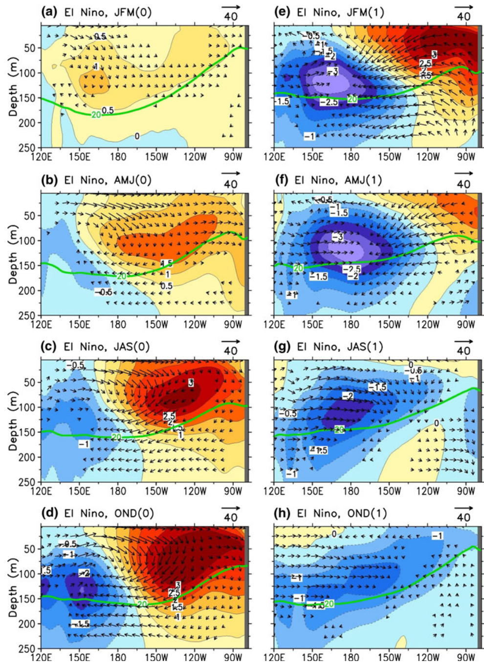
Fig. 10 Seasonal evolution of anomalous temperature (shading) and currents (vectors) in the equatorial ( 1^{\circ}\text{S} – 1^{\circ}\text{N} ) Pacific, and 20^{\circ}\text{C} isotherm (green contour) in the tropical ( 5^{\circ}\text{S} – 5^{\circ}\text{N} ) Pacific. The vertical velocity is amplified according to the scale ratio of longitudinal basin size ( 155^{\circ} ) and depth (250 m). The number in the parenthesis of the subtitle indicates the year of El Niño development
