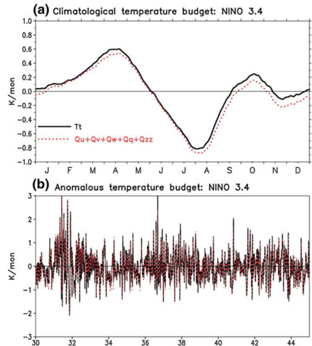
Fig. 3 a Climatological (year 1–60) temperature budget closure at NINO3.4 region ( 5^\circ\text{S} – 5^\circ\text{N} , 170^\circ – 120^\circ\text{W} ). b Anomalous temperature budget closure that is only partially displayed from year 30 to 45. A 7-day running mean is applied in (b) . The correlation coefficient between T_t and the forcing ( Q_u + Q_v + Q_w + Q_{zz} + Q_q ) is 0.995 and 0.97 in (a) and (b) , respectively
