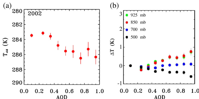
Fig. 8. a) Cloud-top temperature ( T_{\text{cld}} ) of warm clouds versus aerosol optical depth (AOD) in 2002. b) Changes of clear-sky air temperatures with AOD from that of clean air (AOD < 0.2 ) at various pressure levels in the lower and middle troposphere derived from MODIS.
