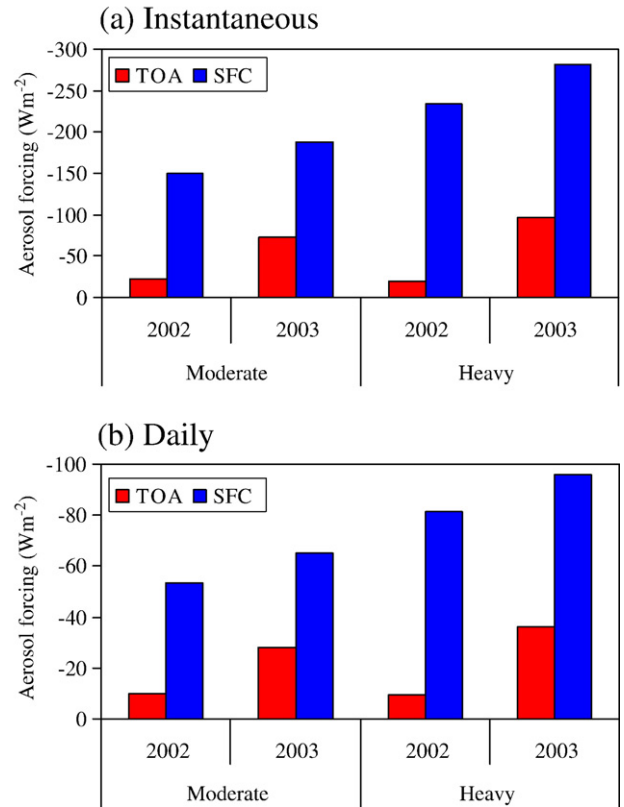
Fig. 18. Changes of (a) instantaneous (1:30 p.m. local time) and (b) daily solar radiative forcing at the top of atmosphere (TOA) and the surface for moderate (AOD=0.55) and heavy (AOD=0.95) smoke conditions and associated changes of warm clouds based on the aerosol-cloud relationship obtained from MODIS data. The aerosol single-scattering albedo and asymmetry factors are taken from AERONET measurements. The aerosol is assumed to be uniformly distributed in the lowest 2 km layer. Clear-sky and cloudy-sky fluxes are calculated separately and then weighted by clear-sky fraction and cloudy-sky fraction to derive average fluxes. For cloudy-sky calculations, the same amount of aerosol as in the clear-sky is assumed to present beneath the cloud layer. AOD=0.1 is an assumed background for deriving the aerosol forcing.
