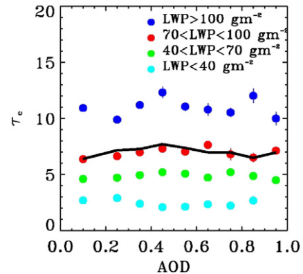
Fig. 9. Water cloud optical depth ( \tau_c ) versus aerosol optical depth (AOD) in 2002. The data are stratified with liquid water path (LWP) and the black line denotes the overall changes for all ranges of LWP.
