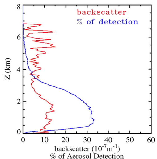
Fig. 17. Detection frequency of aerosol layers and the average aerosol backscatter measured by the Geoscience Laser Altimeter System (GLAS) during September 25–November 19, 2003.
