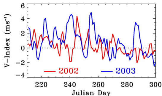
Fig. 2. Comparisons of monsoon index (i.e., V-index) in the Amazon basin between 2002 and 2003. The V-index is defined as the ECMWF daily meridional wind at 925 mb level and averaged over the domain ( 5^{\circ}\text{S} – 5^{\circ}\text{N} , 65^{\circ}\text{W} – 75^{\circ}\text{W} ). A positive and negative value respectively denotes southerly and northerly cross-equatorial flow regime.
