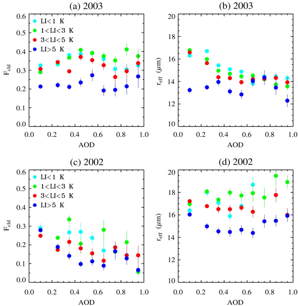
Fig. 15. Changes of cloud fraction ( F_{\text{cld}} ) (a, c) and cloud-top effective radius ( r_{\text{eff}} ) (b, d) with aerosol optical depth (AOD) for 2003 (a, b) and 2002 (c, d). The data are stratified by the MODIS-derived lifted index (LI).
