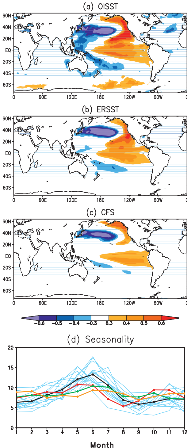
FIG. 1. Spatial patterns of SST associated with the first EOF of monthly-mean SST over the North Pacific (20°–65°N, 125°E–100°W) based on the (a) OISST data during 1982–2010, (b) ERSST during 1861–2010, and (c) the ensemble average of 16 leading EOFs for individual 30-yr segments from the 480-yr CFS coupled run; and (d) seasonal distribution of the percentage variance of PC time series with red for the OISST, green for the ERSST, orange for the PDO index (1900–2010; Mantua et al. 1997), light blue for
