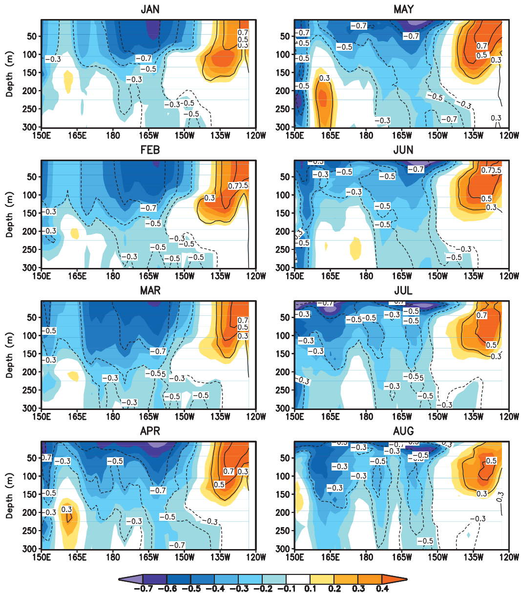
FIG. 3. As in Fig. 2, but based on 29-yr (1982–2010) ocean temperature from the GODAS and the first EOF of North Pacific SST from the OISST.
