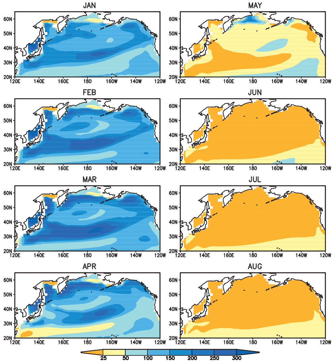
FIG. 4. Monthly climatology of the MLD (m) in the North Pacific derived from the CFS coupled run ensemble averaged over sixteen 30-yr segments for months from January to August.
