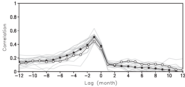
FIG. 8. Lag correlations between the PC time series of the first EOF of monthly 1000-hPa zonal wind and SST over the North Pacific in the CFS coupled run for each 30-yr period (gray) and ensemble average (black line with filled circles) of the 16 correlation coefficients at different lags and those using 29-yr 1000-hPa zonal wind from GR-2 and OISST (black line with open circles). Negative (positive) lag means the 1000-hPa zonal wind leading (lagging) the SST.
