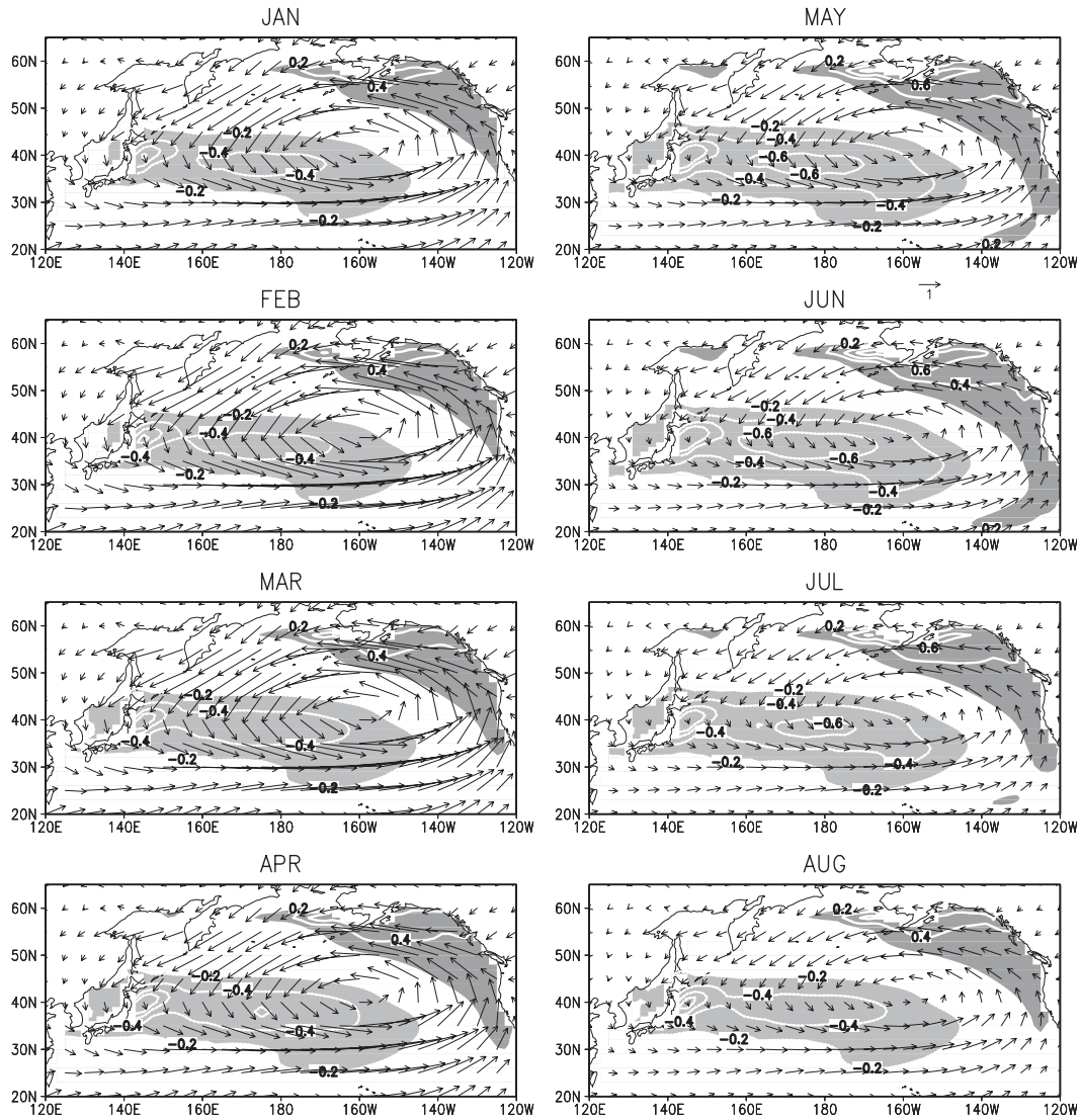
FIG. 6. Regression patterns of 1000-hPa wind (vectors, \text{m s}^{-1} ) and SST (shadings, ^{\circ}\text{C} ) anomalies in the CFS associated with departures of one standard deviation of the PC time series of the first EOF of 1000-hPa zonal wind and SST anomalies over the North Pacific, respectively. The regressions are performed over the 30-yr period and all months, but values of one standard deviation of the PC time series are calculated for individual months from January to August. The results are shown based on a 16-member ensemble. Contour interval is 0.2^{\circ}\text{C} with negative values dashed and zero contours omitted. Dark (light) shadings indicate positive (negative) SST anomalies exceeding 0.2^{\circ}\text{C} .
