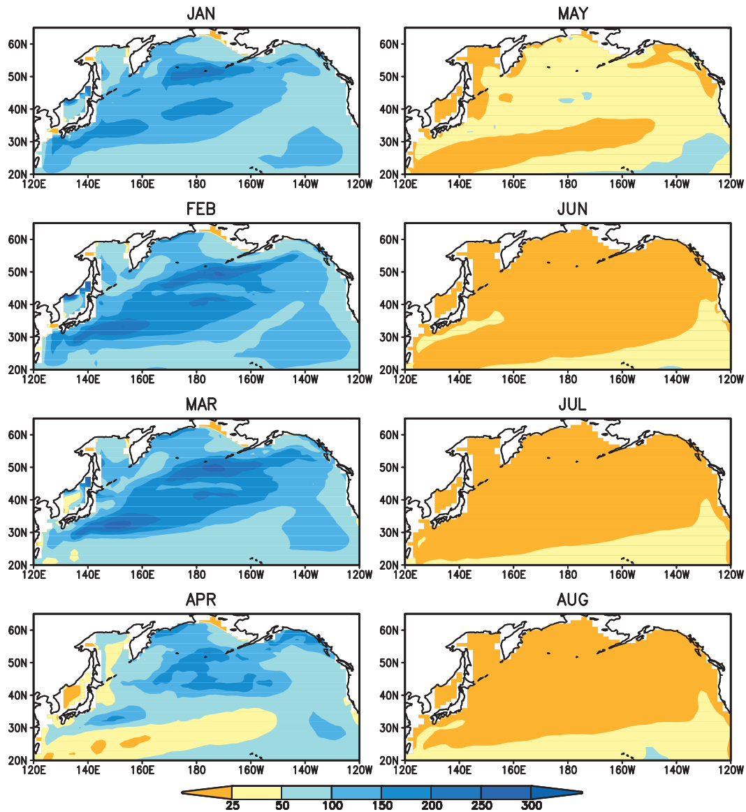
FIG. 5. As in Fig. 4, but based on 29-yr (1982–2010) GODAS data.
