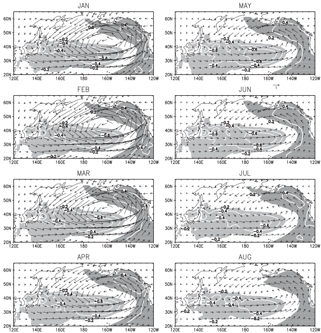
FIG. 7. As in Fig. 6, but based on 29-yr (1982–2010) 1000-hPa wind from GR-2 and OISST.
