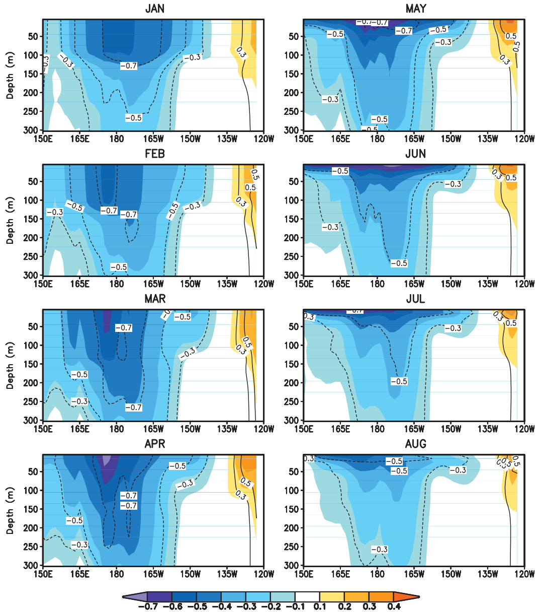
FIG. 2. PDO-related monthly ocean temperature anomalies (shading, ^{\circ}\text{C} ) and correlation (contour) with the PDO PC time series at 37^{\circ}\text{N} across the North Pacific in the CFS. The anomalies are obtained by regressing ocean temperature anomaly vs the PC time series of the first EOF of North Pacific SST in individual 30-yr segments. The anomalies are based on the ensemble average of 16 members and are associated with fluctuations of one standard deviation in the PC time series for months from January to August. The correlation coefficients are also based on the ensemble average of the 16 members. Contours are \pm 0.3 , \pm 0.5 , and \pm 0.7 with negative contours dashed.
