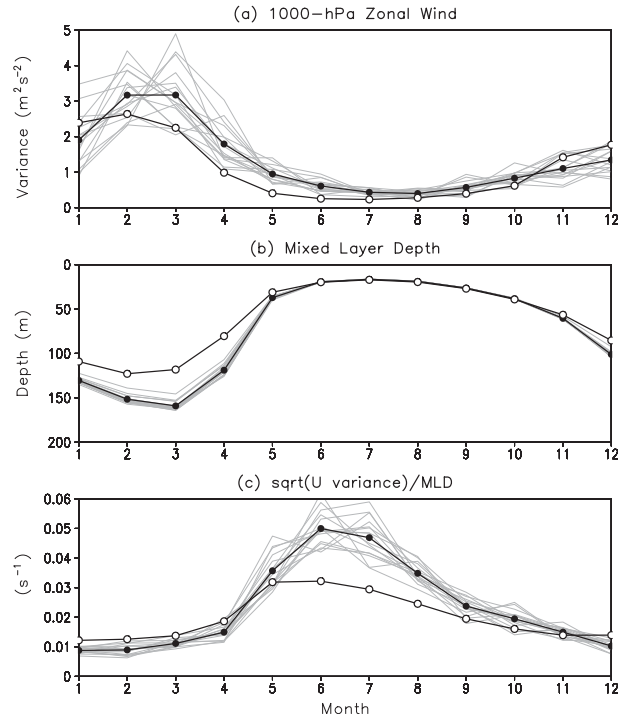
FIG. 9. Seasonal variations of area-averaged ( 20^{\circ} – 65^{\circ} N, 125^{\circ} E– 120^{\circ} W) (a) monthly-mean variance of the 1000-hPa zonal wind anomaly associated with the first EOF, (b) climatological MLD, and (c) square root of the zonal wind variance in month N - 1 divided by the MLD in month N . Gray lines are for 16 individual members from the CFS, black lines with filled circles for ensemble means, and black lines with open circles for observations (GR-2 and GODAS).
