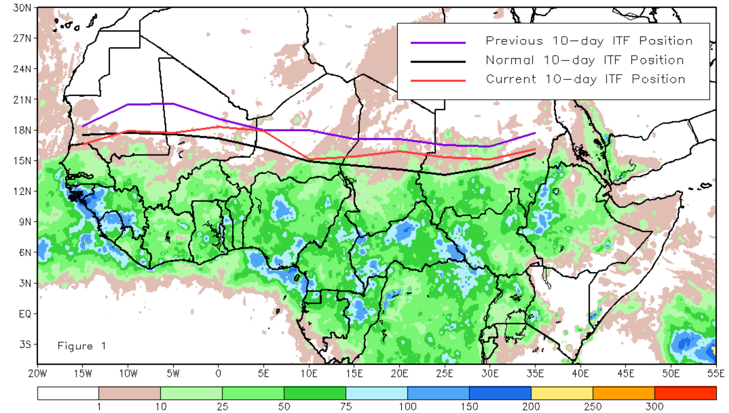
Current vs. Normal Dekadal ITF Position and RFE Accumulated Precipitation (mm) September 2023, Dekad 3
