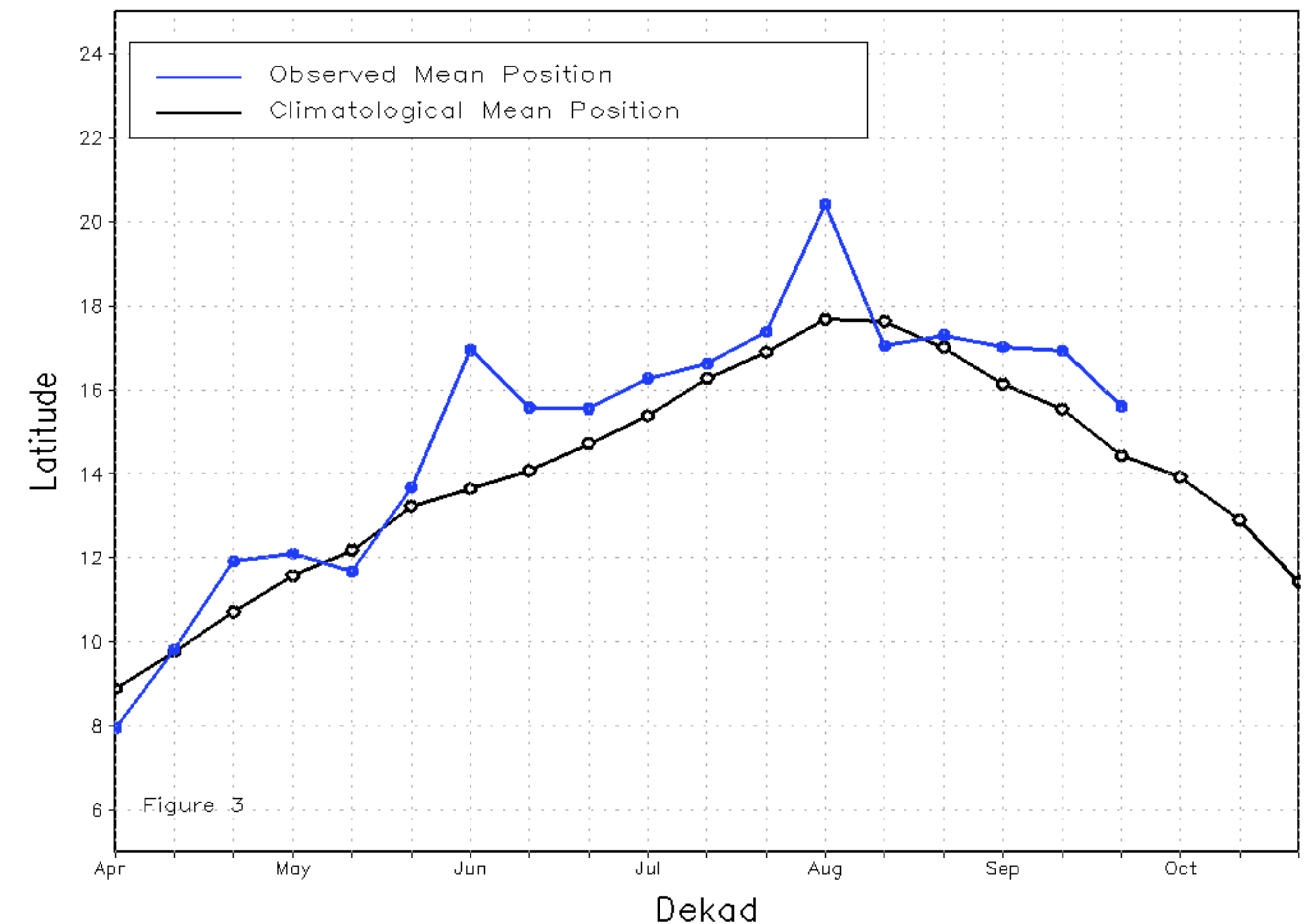
Mean Eastern Portion of the ITF: Averaged 20E to 35E As of: September 2023, Dekad 3
