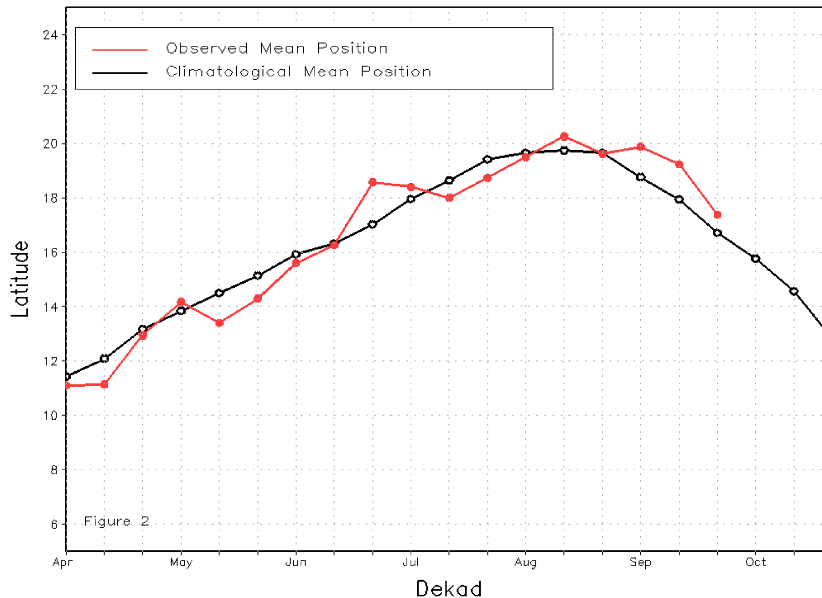
Mean Western Portion of the ITF: Averaged 10W to 10E As of: September 2023, Dekad 3
