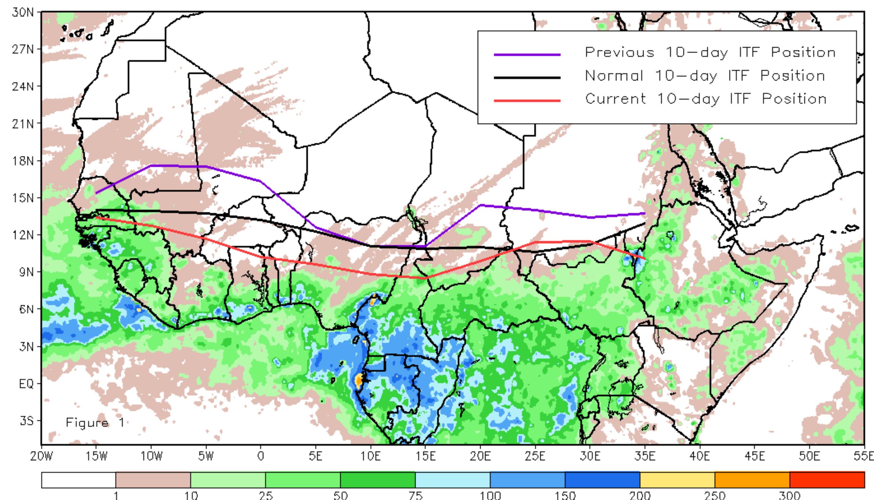
Current vs. Normal Dekadal ITF Position and RFE Accumulated Precipitation (mm) October 2022, Dekad 3
