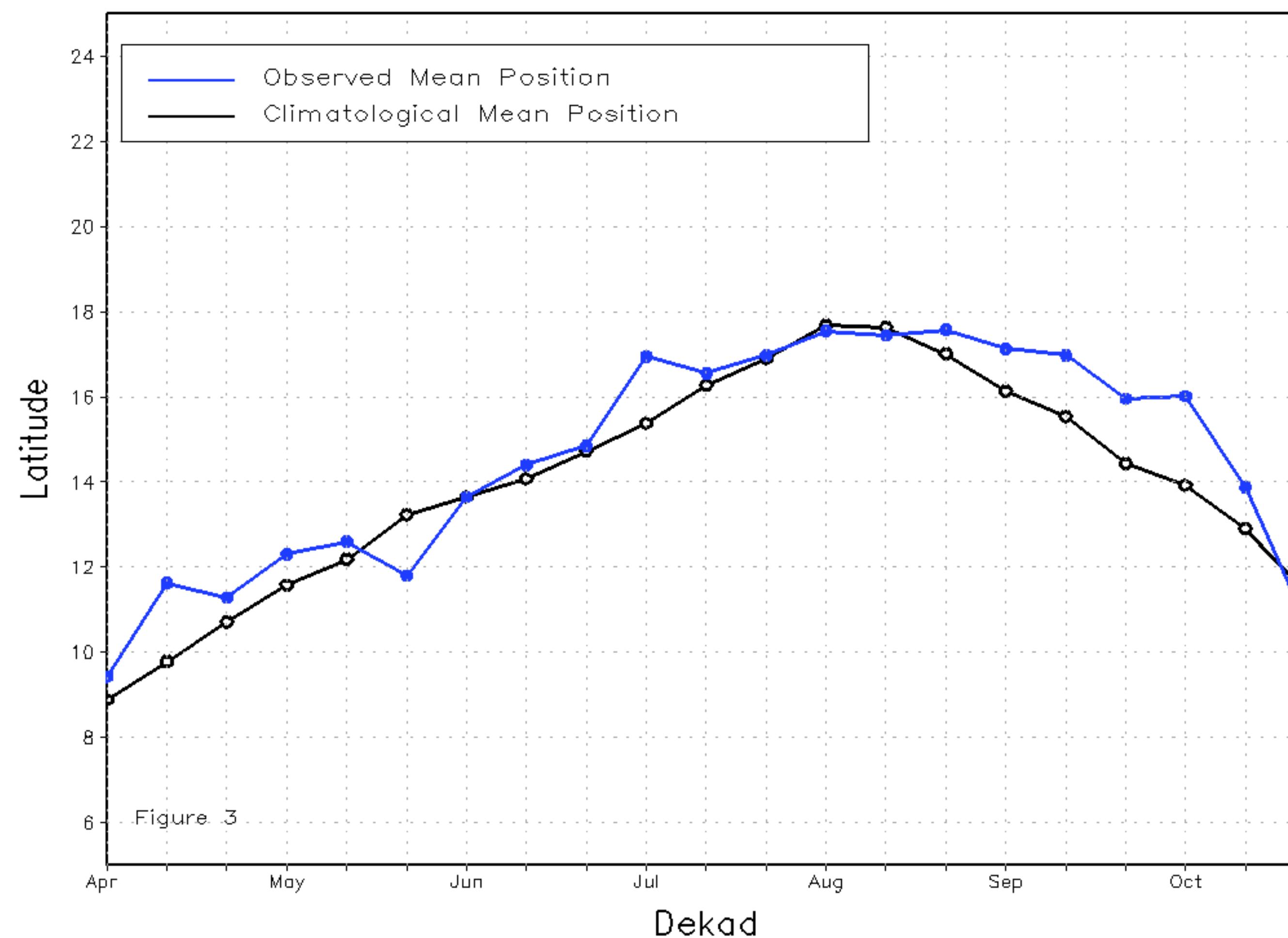
Mean Eastern Portion of the ITF: Averaged 20E to 35E As of: October 2022, Dekad 3
