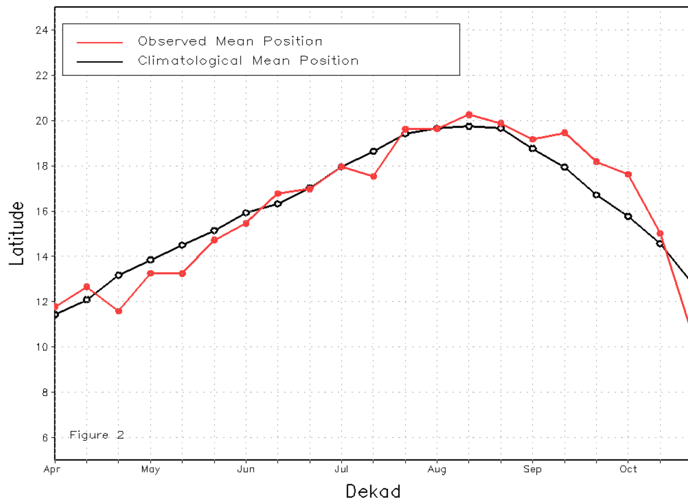
Mean Western Portion of the ITF: Averaged 10W to 10E As of: October 2022, Dekad 3
