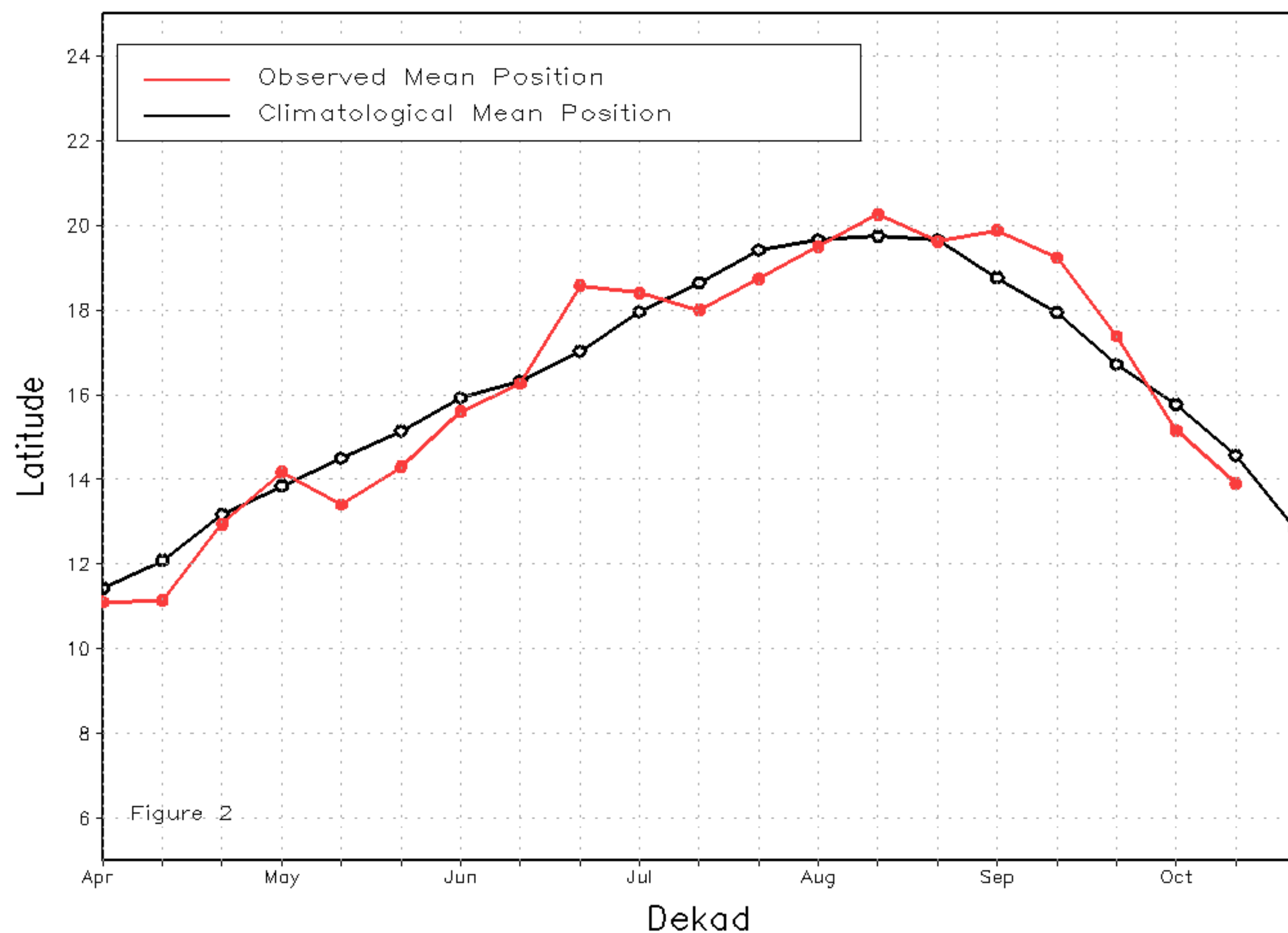
Mean Western Portion of the ITF: Averaged 10W to 10E As of: October 2023, Dekad 2
