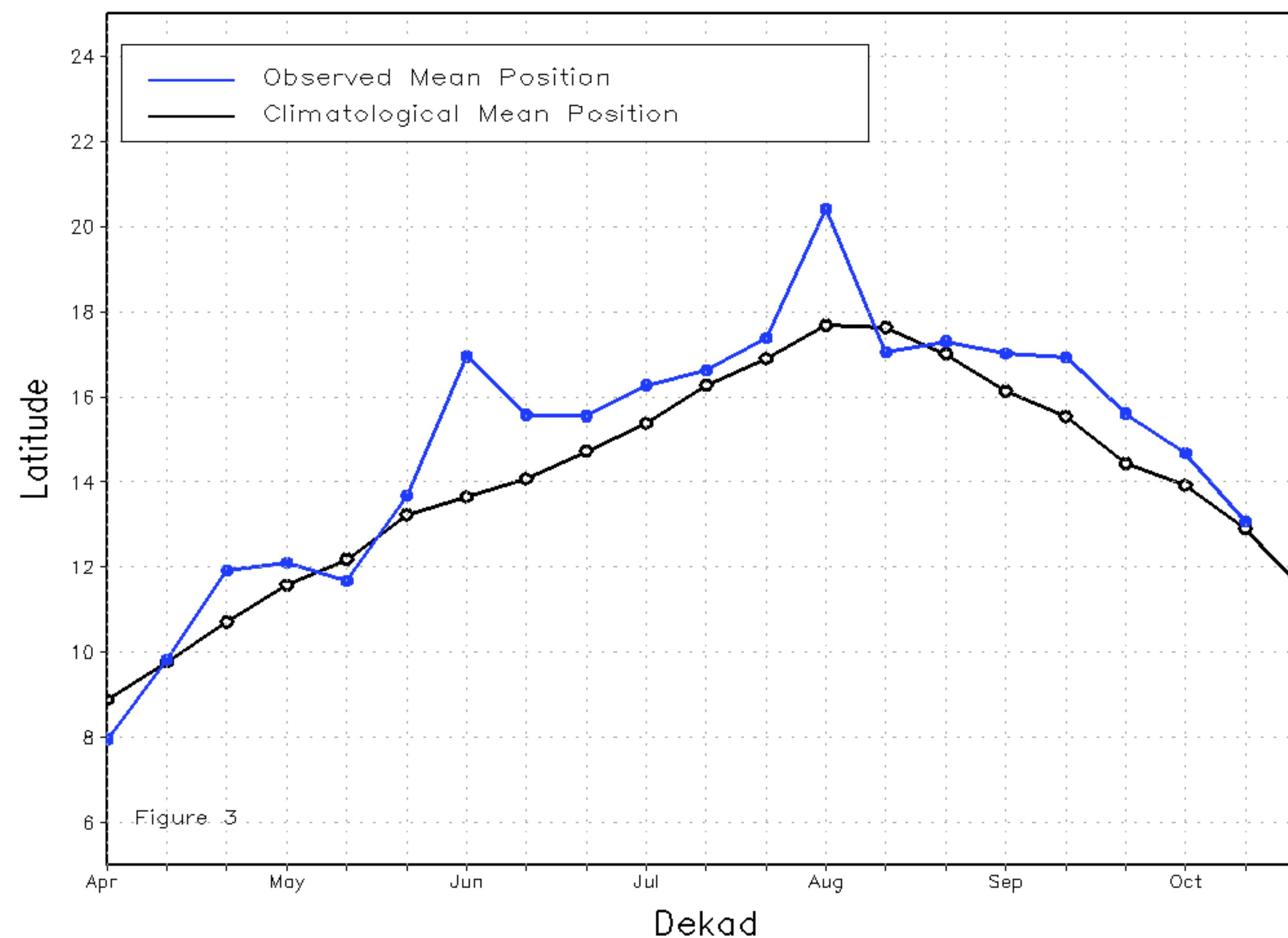
Mean Eastern Portion of the ITF: Averaged 20E to 35E As of: October 2023, Dekad 2
