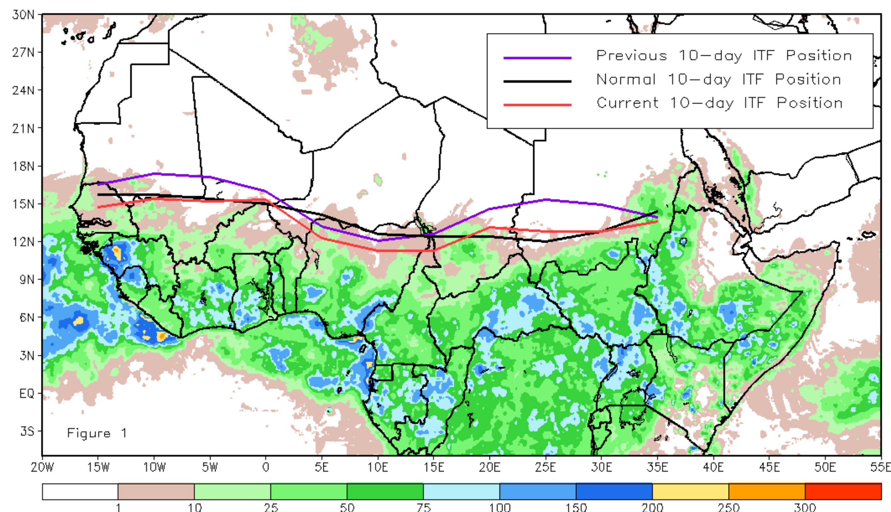
Current vs. Normal Dekadal ITF Position and RFE Accumulated Precipitation (mm) October 2023, Dekad 2
