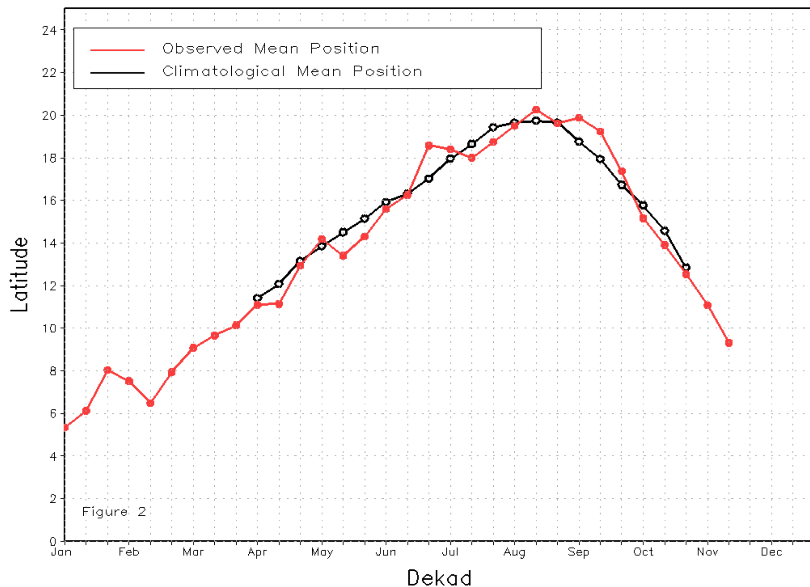
Mean Western Portion of the ITF: Averaged 10W to 10E As of: November 2023, Dekad 2
