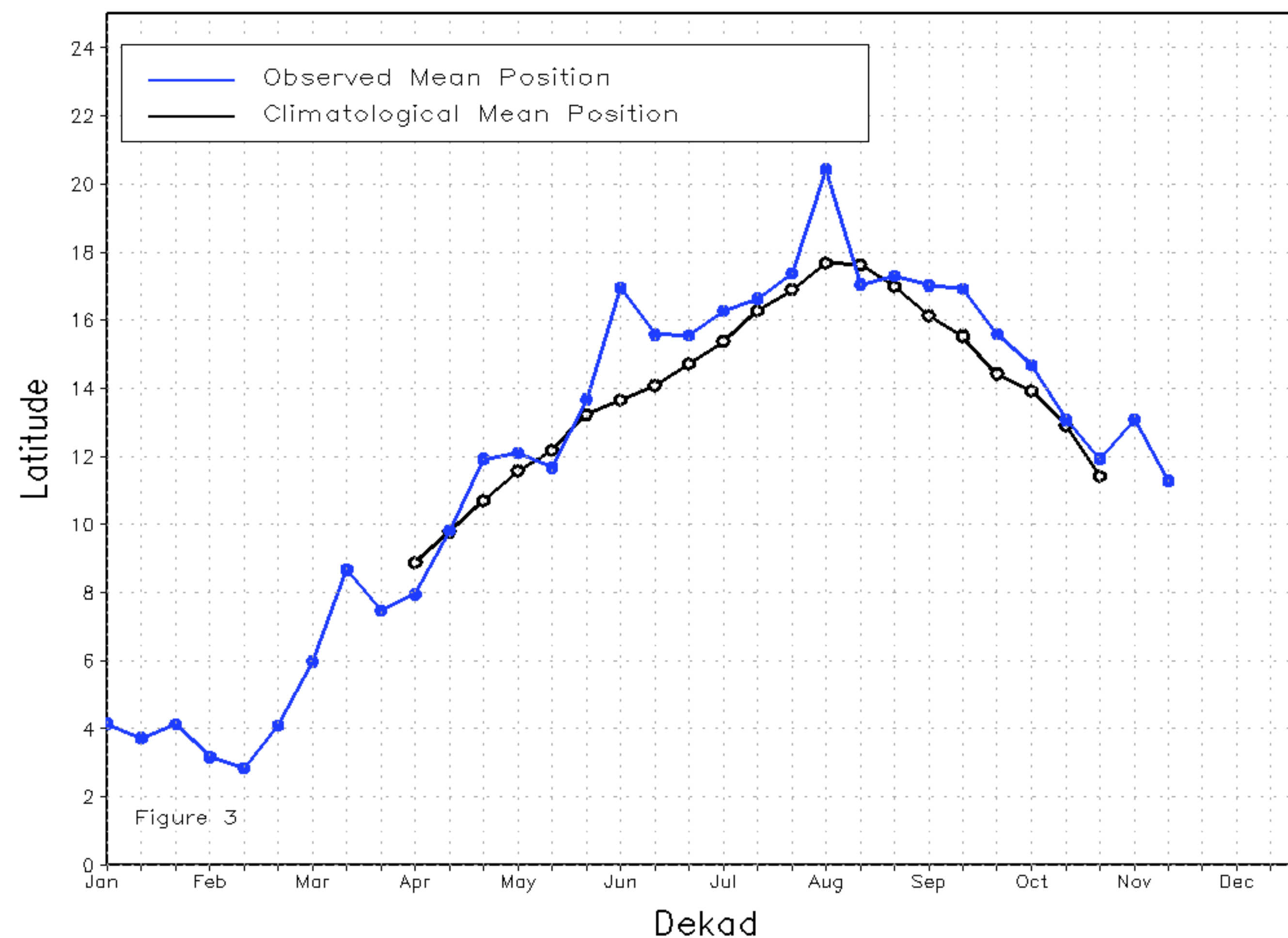
Mean Eastern Portion of the ITF: Averaged 20E to 35E As of: November 2023, Dekad 2
