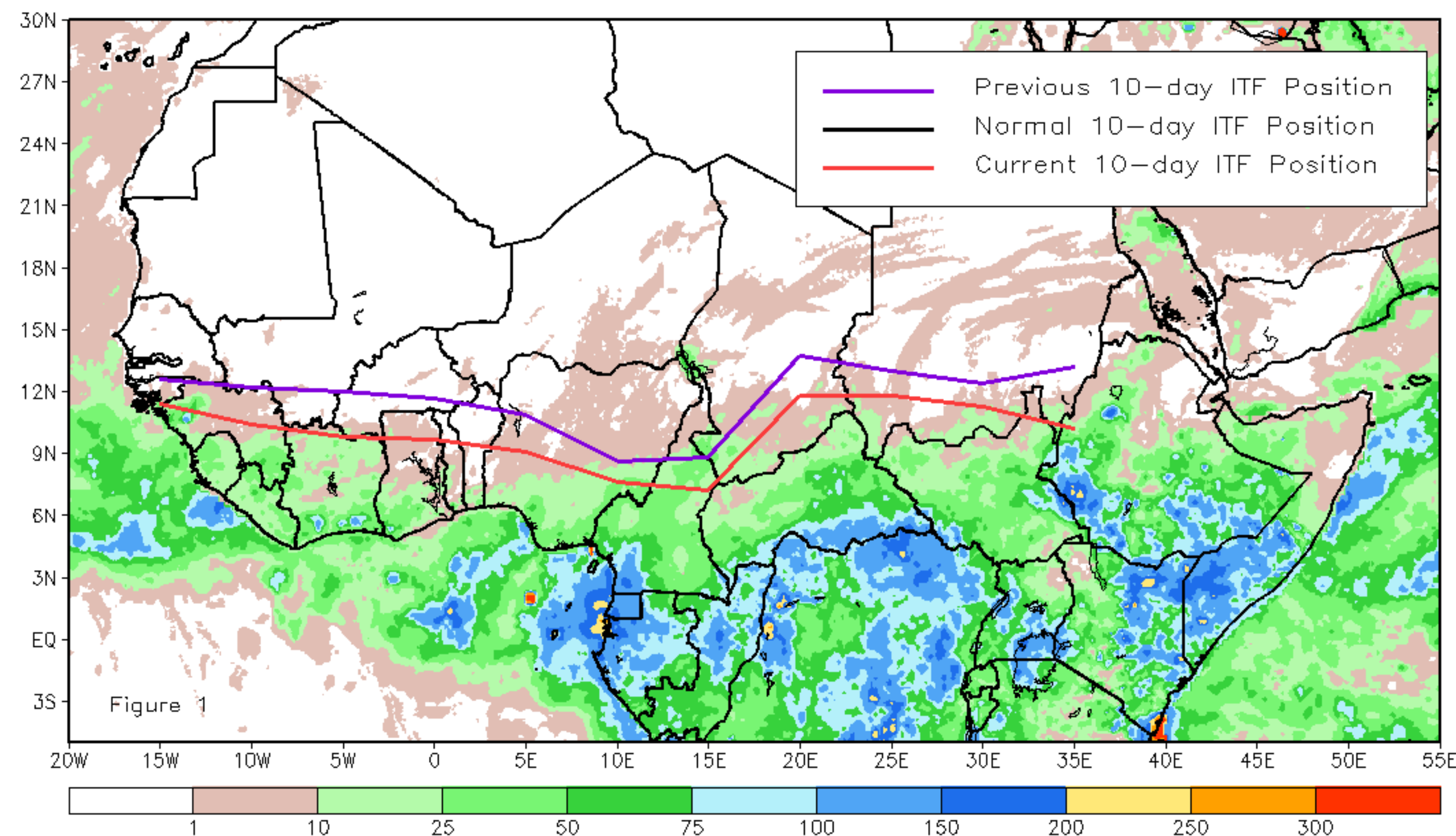
Mean Eastern Portion of the ITF: Averaged 20E to 35E As of: November 2023, Dekad 2
