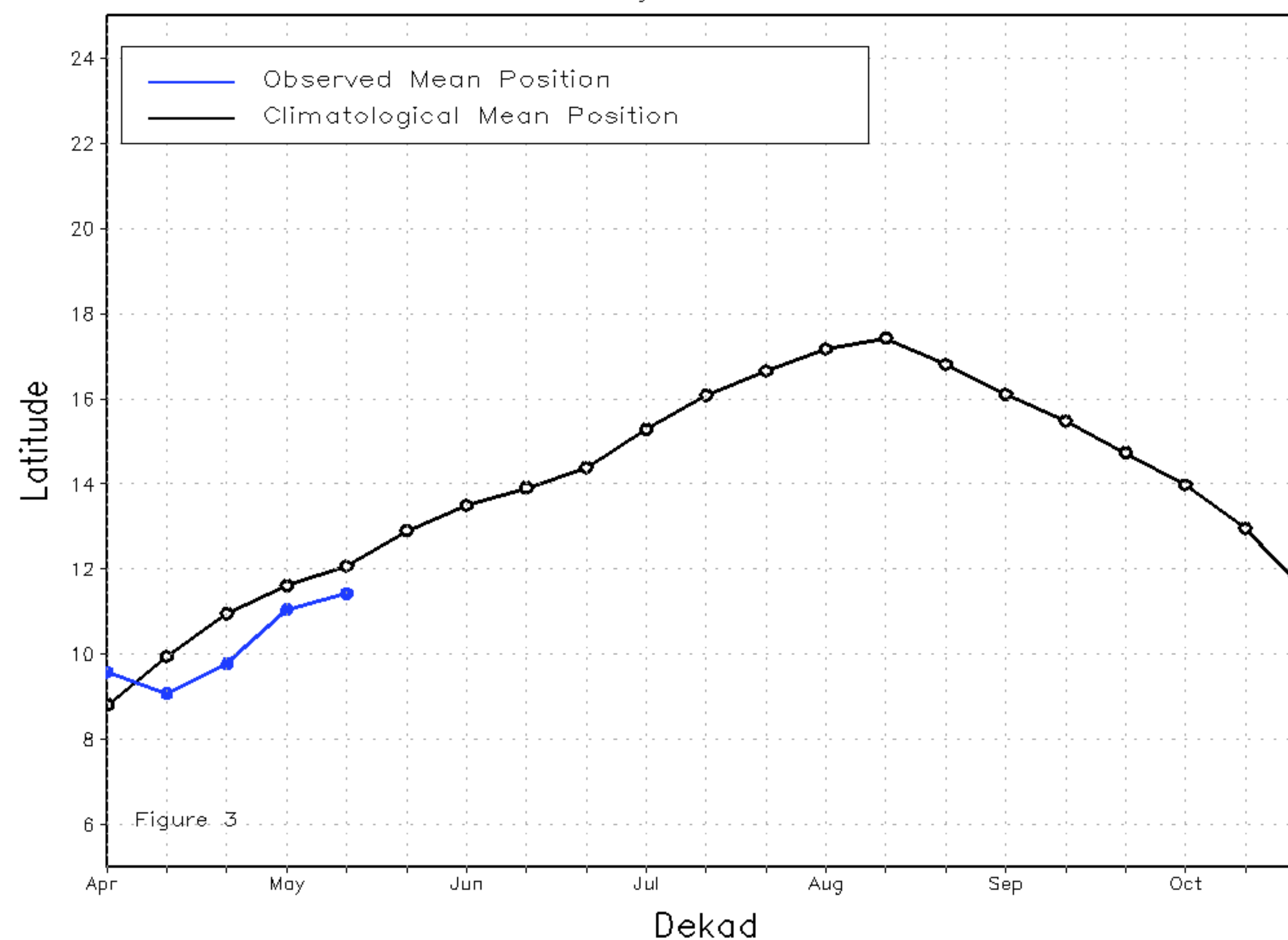
Mean Eastern Portion of the ITF: Averaged 20E to 35E As of: May 2020, Dekad 2
