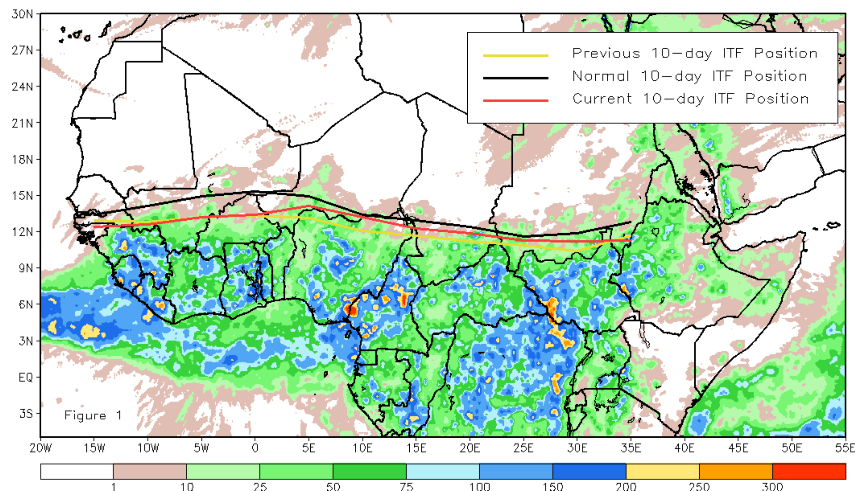
Current vs. Normal Dekadal ITF Position and RFE Accumulated Precipitation (mm) May 2020, Dekad 2
