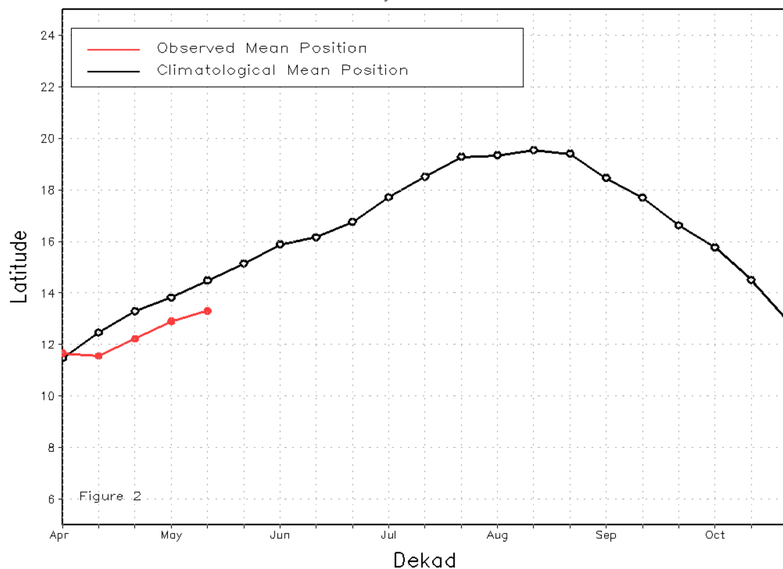
Mean Western Portion of the ITF: Averaged 10W to 10E As of: May 2020, Dekad 2
