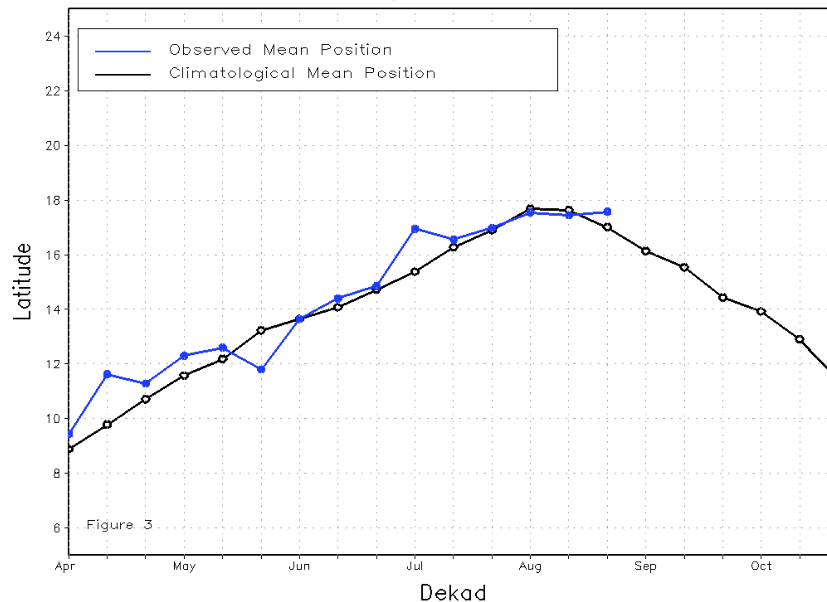
Mean Eastern Portion of the ITF: Averaged 20E to 35E As of: August 2022, Dekad 3
