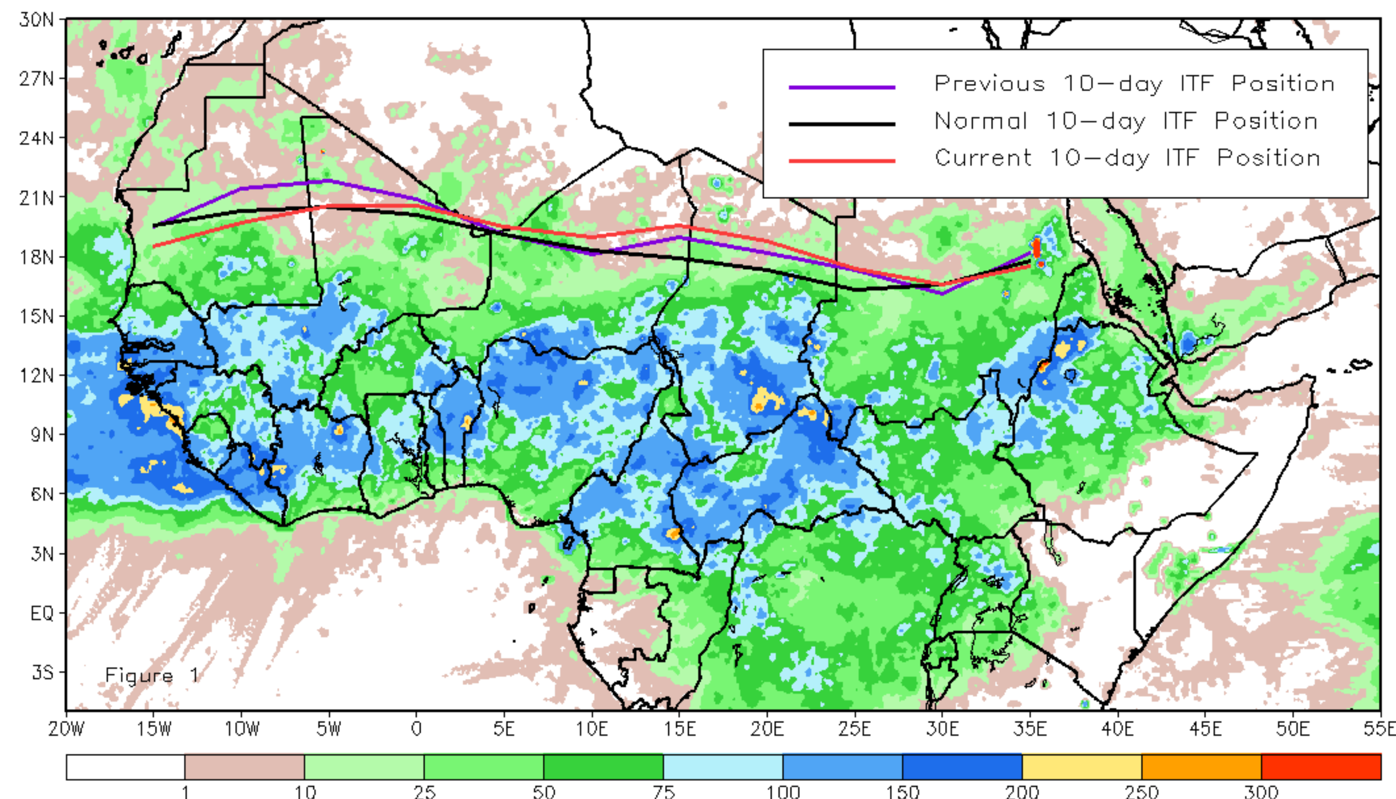
Current vs. Normal Dekadal ITF Position and RFE Accumulated Precipitation (mm) August 2022, Dekad 3
