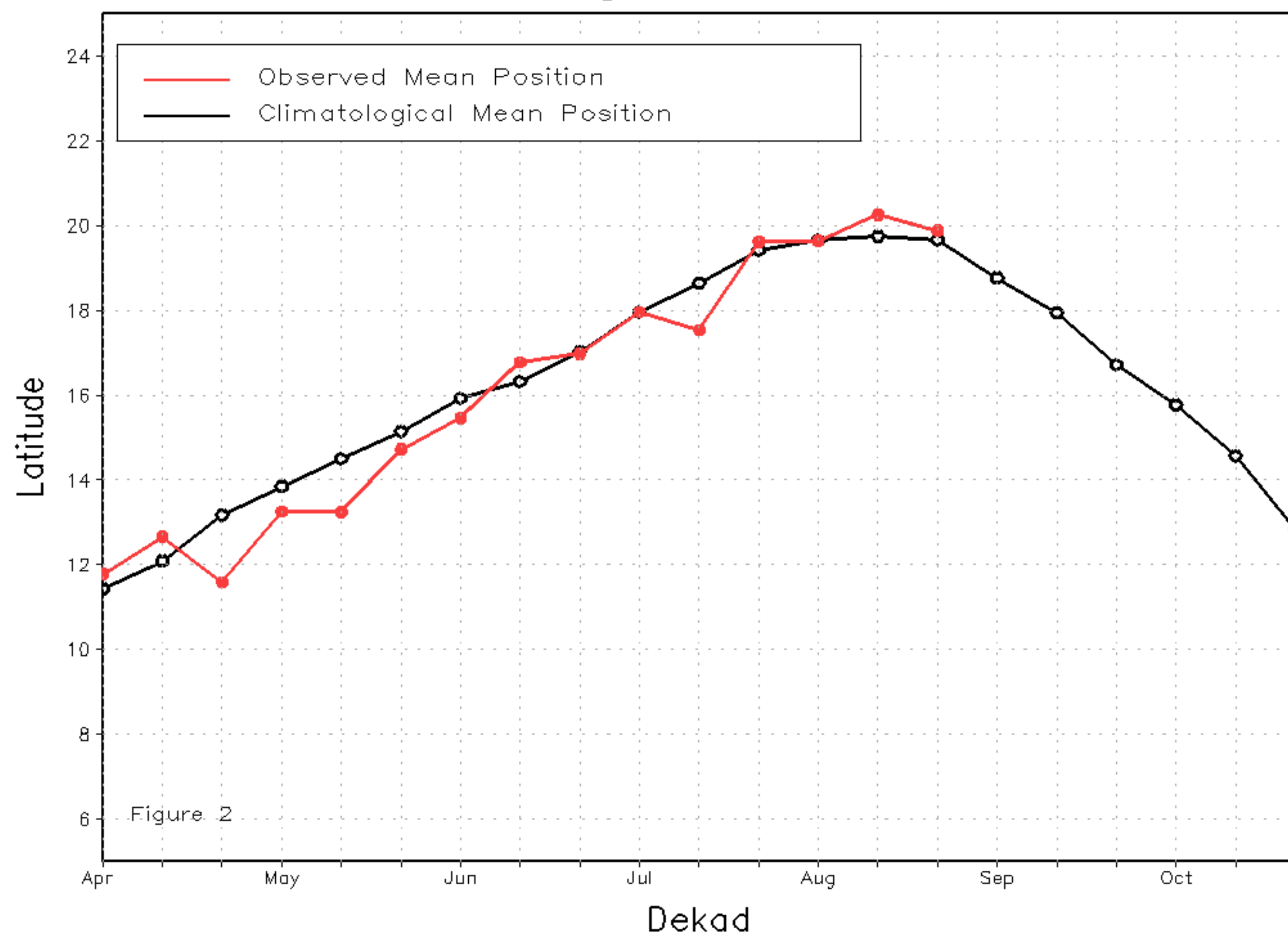
Mean Western Portion of the ITF: Averaged 10W to 10E As of: August 2022, Dekad 3
