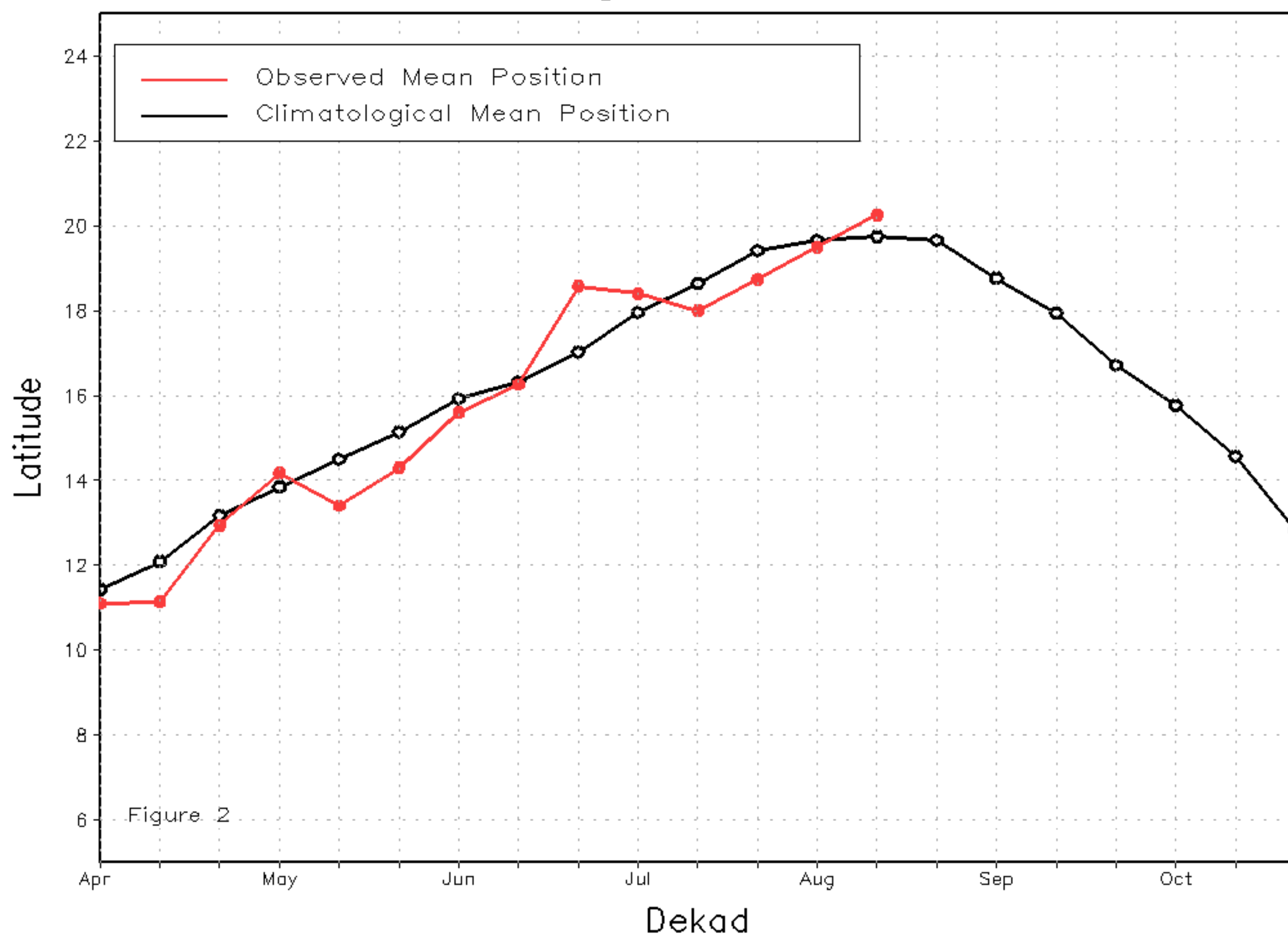
Mean Western Portion of the ITF: Averaged 10W to 10E As of: August 2023, Dekad 2
