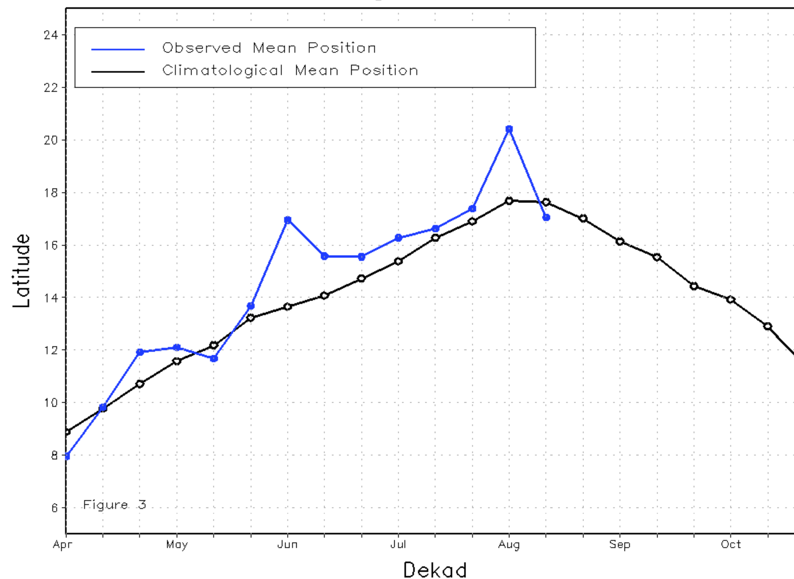
Mean Eastern Portion of the ITF: Averaged 20E to 35E As of: August 2023, Dekad 2
