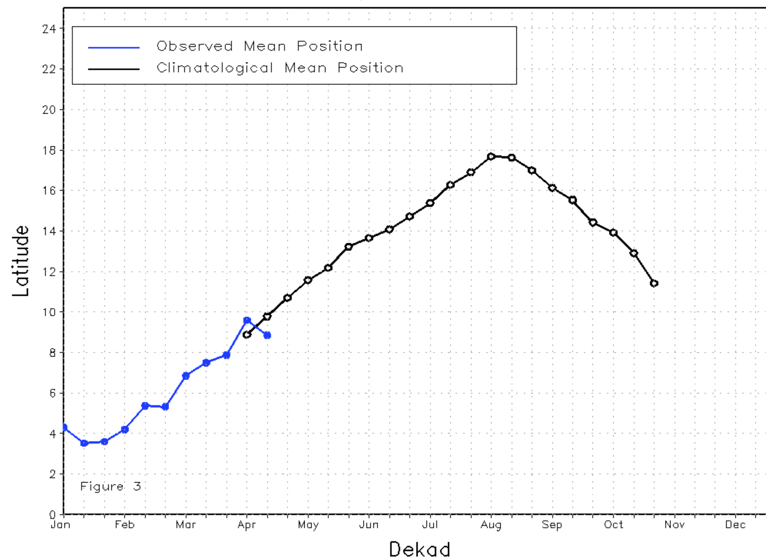
Mean Eastern Portion of the ITF: Averaged 20E to 35E As of: April 2024, Dekad 2
