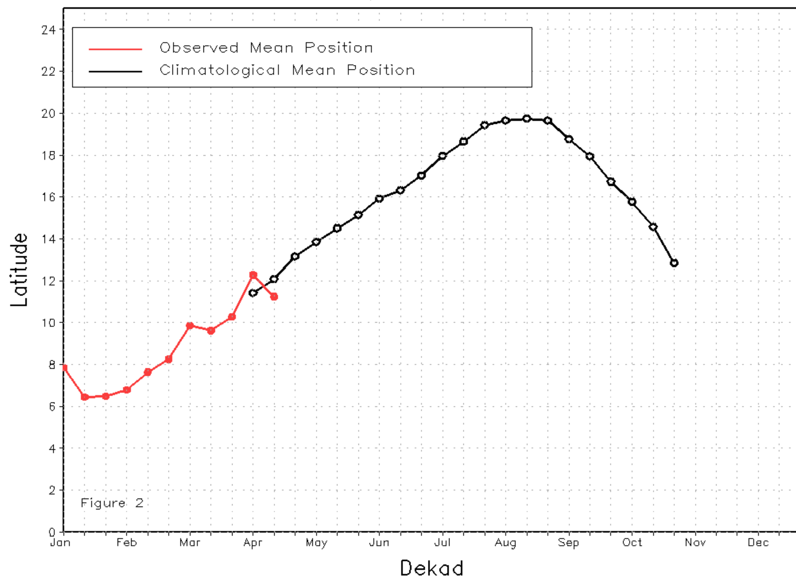
Mean Western Portion of the ITF: Averaged 10W to 10E As of: April 2024, Dekad 2
