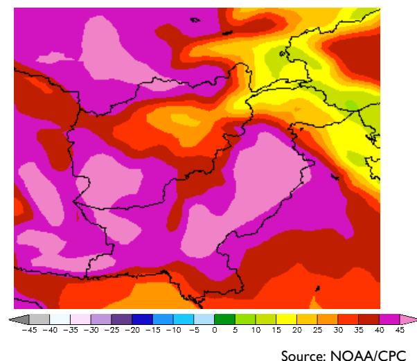
Figure 3. Extreme Maximum Temperature (°C) for July 27 – August 2, 2009.
