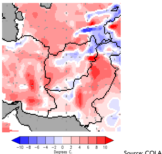
Figure 2. Temperature Anomaly for July 27 – August 2, 2009.
