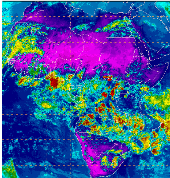
IR Satellite Image (valid 1530z March 01, 2016)
