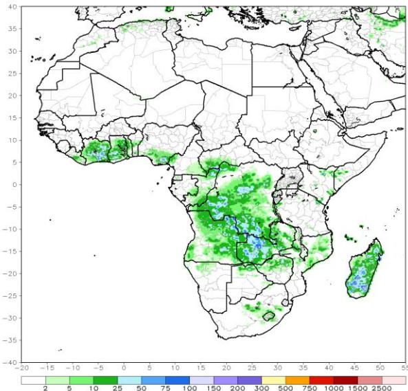
RFE2 Daily Total Rainfall (mm) Period: 29Feb2016
