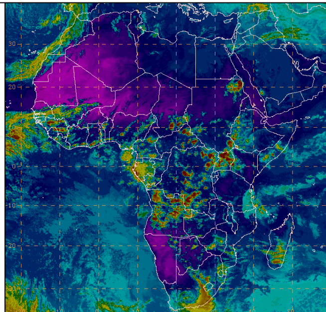
IR Satellite Image (valid 15520Z of 25 October 2013)
