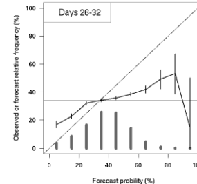
l) Reliability diagram: event positive precip anom for week 4: Issued MAM - 2015-2016-2017 fcst
