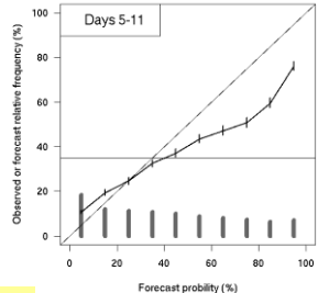
i) Reliability diagram: event positive precip anom for week 1: Issued MAM - 2015-2016-2017 fcst
