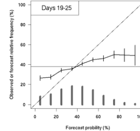
c) Reliability diagram: event positive precip anom for week 18-24 APR: Issued 31 MAR - 1996-2015 hind
