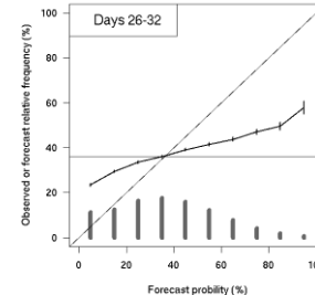
h) Reliability diagram: event positive precip anom for week 4: Issued MAM - 1996-2015 hind
