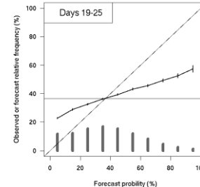
g) Reliability diagram: event positive precip anom for week 3: Issued MAM - 1996-2015 hind
