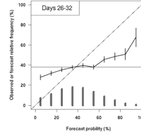
d) Reliability diagram: event positive precip anom for week 18-24 APR: Issued 24 MAR - 1996-2015 hind
