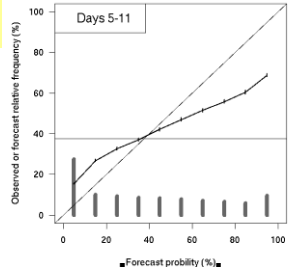
e) Reliability diagram: event positive precip anom for week 1: Issued MAM - 1996-2015 hind
