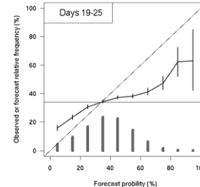
k) Reliability diagram: event positive precip anom for week 3: Issued MAM - 2015-2016-2017 fcst
