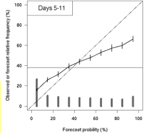
a) Reliability diagram: event positive precip anom for week 18-24 APR: Issued 14 APR - 1996-2015 hind
