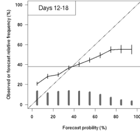
b) Reliability diagram: event positive precip anom for week 18-24 APR: Issued 7 APR - 1996-2015 hind
