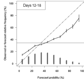
j) Reliability diagram: event positive precip anom for week 2: Issued MAM - 2015-2016-2017 fcst
