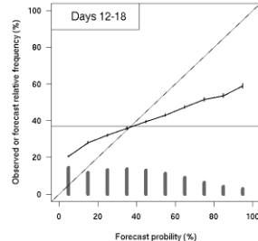
f) Reliability diagram: event positive precip anom for week 2: Issued MAM - 1996-2015 hind
