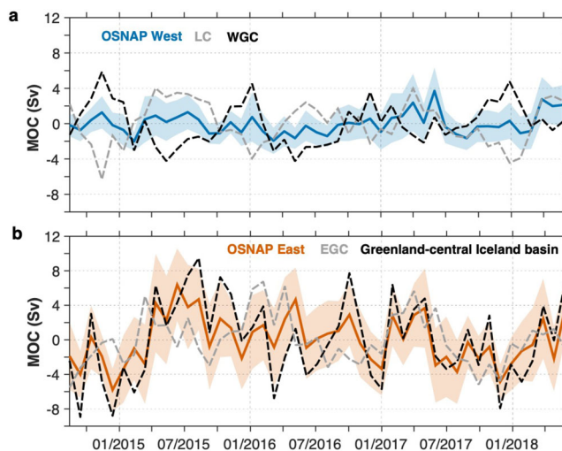
Fig. 4 Components of overturning variability. a OSNAP West Meridional Overturning Circulation (MOC) anomalies: overturning derived from the Labrador Sea array (blue; shading indicates uncertainty as shown in Fig. 2); MOC variability arising from time-varying density and velocity anomalies in the Labrador Current (LC; light gray) computed with time-mean velocities/densities at the West Greenland Current (WGC) boundary, and MOC variability arising from density and velocity anomalies in the WGC (black) computed with time-mean velocities/densities at the LC boundary. b OSNAP East MOC anomalies: overturning derived from the OSNAP East array (red; shading indicates uncertainty as shown in Fig. 2); MOC variability arising from time-varying density and velocity in the region between Greenland and mid-Iceland basin (black) computed with time-mean velocities/densities at the eastern boundary, and MOC variability arising from density and velocity anomalies in the East Greenland Current (EGC; light gray) computed with time-mean velocities/densities everywhere else. For the reconstruction based on the time-varying data at the western boundary (light gray line), the MOC is defined as the minimum of the stream function integrated from the bottom to the sea surface in density space (sign has been changed for comparisons).
